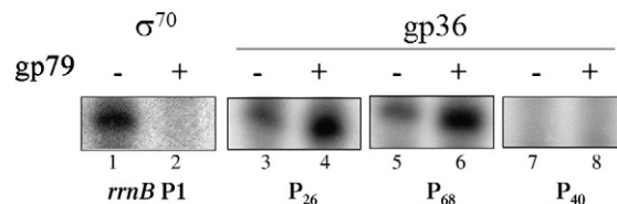
Fig. 7. PhiEco32 gp79 activates gp36-dependent transcription in vitro . The results of in vitro transcription by indicated E. coli RNAP holoenzymes in the presence or in the absence of gp79 are shown. In lanes 1 and 2, a DNA fragment containing a strong \sigma^{70} -dependent rrnB P1 promoter was used as template.
