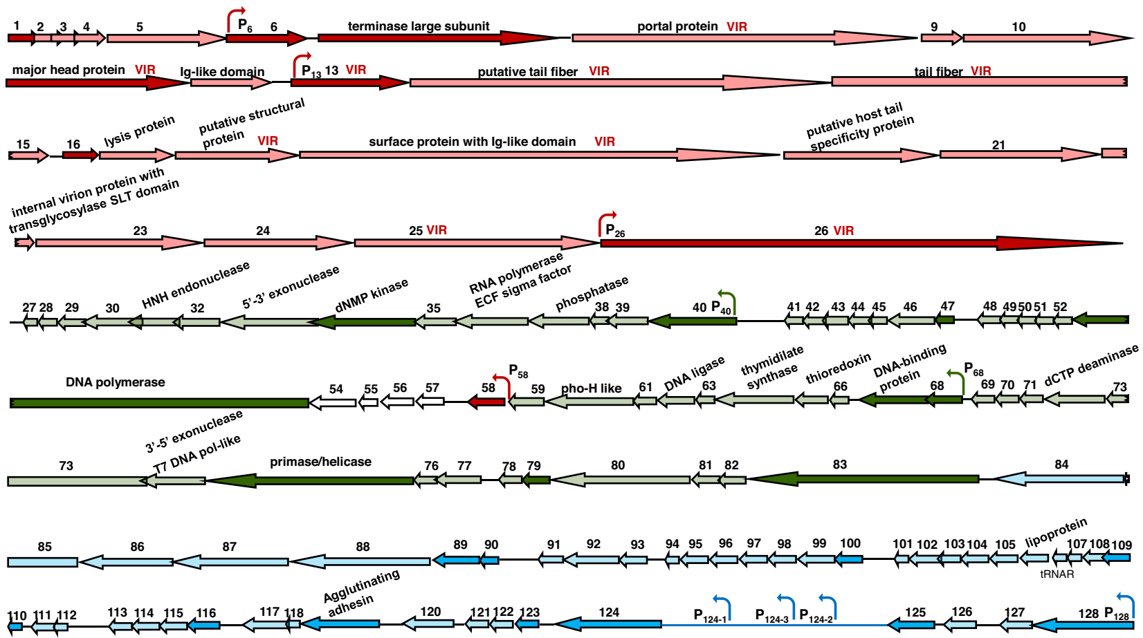
Fig. 1. Temporal classes of bacteriophage phiEco32 genes. The genome of phiEco32 phage is schematically presented. Arrows represent annotated genes; the direction of the arrow indicates the direction of transcription. Intergenic regions of 60 bp or more are shown as a plain line. Genes belonging to different temporal classes are indicated in blue (early genes), green (middle genes), and red (late genes). Genes assigned to specific temporal classes based on experimental data (primer extension and/or macroarray analysis) are shown in dark colors. Genes assigned to specific temporal classes based on a predicted operonic structure of the phiEco32 genome are shown in light colors. Genes for which no assignments can be made based on data available are shown in white. Promoters are shown as bent arrows; the color of a promoter arrow indicates its temporal class. The putative functions of phiEco32 genes, when known, are indicated. "Vir" indicates proteins present in the phiEco32 virion. 2
