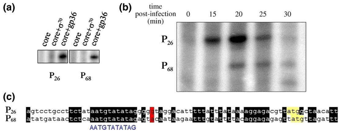
Fig. 4. Experimental identification of gp36-dependent phiEco32 promoters. (a) The results of in vitro transcription by the E. coli RNAP core enzyme in the presence of \sigma^{70} or gp36 from DNA fragments corresponding to intergenic regions from phiEco32 genes 26 and 68. (b) Total RNA isolated from cells collected at various time points postinfection and subjected to primer extension analysis with primers annealing within genes 26 and 68. The reaction products were separated in a 6% denaturing polyacrylamide gel and visualized using PhosphorImager. (c) Comparison of DNA sequences upstream of experimentally determined transcription start points for P 26 and P 68 . The transcription start point is shown in red; annotated translation start codons are highlighted in yellow. Identical bases in compared sequences are shown against a black background. A common motif upstream of transcription start points used for bioinformatic searches is shown below the alignment.
