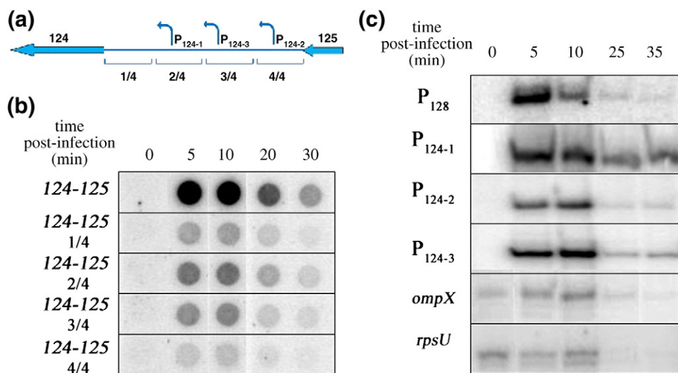
Fig. 3. Mapping of early phiEco32 promoters. (a) Schematic presentation of the 124–125 intergenic region. The relative positions of fragments 1/4, 2/4, 3/4, and 4/4 used as probes on the array are shown below. Bent leftward arrows represent early promoters P_{124-1} , P_{124-2} , and P_{124-3} . (b) The representative result of an experiment with an array of fragments of the 124–125 intergenic region hybridizing to the total RNA prepared from cells collected at various time points postinfection. (c) The results of the primer extension analysis of total RNA prepared from cells collected at various time points postinfection using primers designed to reveal transcription from individual phiEco32 early promoters and selected host promoters.
