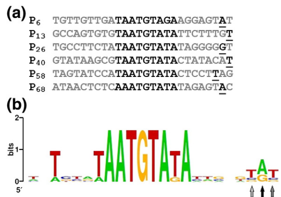
Fig. 5. Bioinformatic search for additional gp36-dependent promoters. Sequences upstream of phiEco32 genes 6, 13, 26, 40, 58, and 68 are presented with a shared motif indicated in black. Experimentally determined in vivo transcription initiation start points (as judged by primer extension) are underlined. Below: A logo representation of the gp36 promoters of the phage is shown. The height of a letter indicates the degree of conservation. Upward vertical arrows indicate the positions of transcription start points; the color of the arrow indicates transcription initiation frequency, with black being the highest, white - the lowest.
