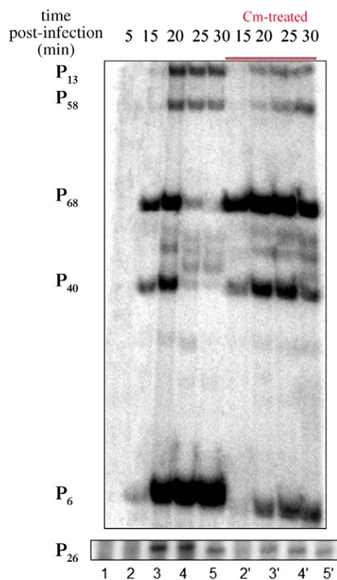
Fig. 6. Kinetics of accumulation of gp36-dependent transcripts during phiEco32 infection. Results of the multiplex primer extension analysis of total RNA extracted from phage-infected cells collected at various time points postinfection are shown. Primer extension reactions on the right-hand side of the figure (lanes 2'–5') were conducted with RNA prepared from infected cells that were subjected to chloramphenicol treatment 12 min postinfection. The reaction products were separated in a 6% denaturing polyacrylamide gel and visualized using PhosphorImager.
